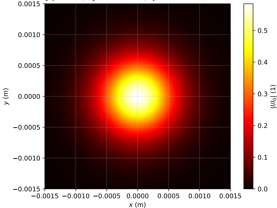
Intensity profile I(x, y, z = 3.423m)/I_0 , \text{Pin}=0.6\text{Pcr} , artificial time
